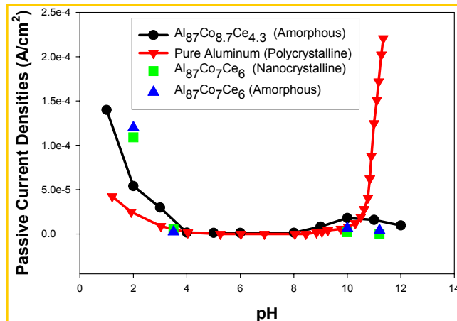
Figure 4. Passive current densities for high purity \text{Al}^{27} and amorphous alloys of the Al-Co-Ce system including heat-treated nanocrystalline material, in solution adjusted to various pH values using concentrated HCl or 1 M NaOH as necessary.
