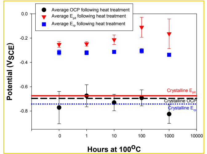
Figure 8. Effect of 100°C isothermal heat treatments on E_{pit} , E_{rp} and OCP values for Al_{87}Co_7Ce_6 alloy when tested in deaerated 0.6 M NaCl after a one hour exposure to solution. Data is compared to fully crystalline Al_{87}Co_7Ce_6 alloy after 550°C isothermal heat treatment.
