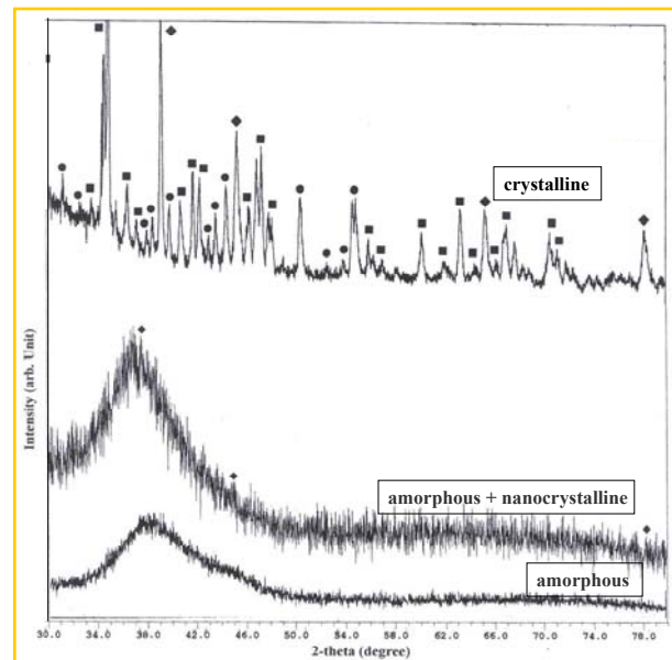
Figure 2. X-ray diffraction patterns ( \text{Cu K}_\alpha radiation at 40 kV and 35 mA) for the melt-spun \text{Al}_{87}\text{Co}_{8.7}\text{Ce}_{4.3} alloy ribbon (52 m/s wheel speed) showing the amorphous microstructure of the as-quenched material the amorphous + nanocrystalline microstructure of the 100 hour 100^\circ\text{C} treatment, and the crystalline microstructure which is developed after a non-isothermal 550^\circ\text{C} heat-treatment.
